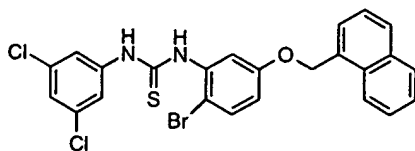
Compound # 33
